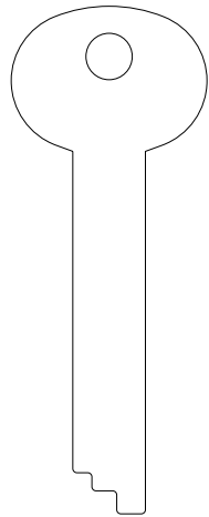
.050" - 1.3mm .350" - 8.9mm 1134
