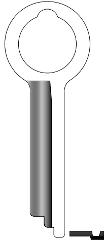
.080" - 2.0mm .350" - 8.9mm 1135
