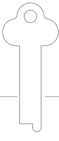
.050" - 1.3mm .375" - 9.5mm 1093
