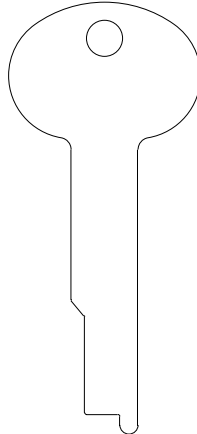
.070" - 1.8mm .280" - 7.1mm 1362
