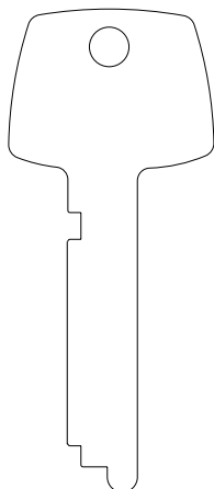
.070" - 1.8mm .330" - 8.4mm 1333
