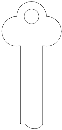
.060" - 1.5mm .380" - 9.7mm 1323
